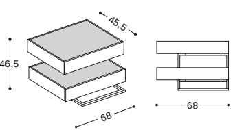
BOSTON B - 2 cassetti / 2 drawers
