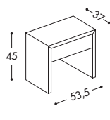
MINORCA 1 cassetto / 1 drawer
